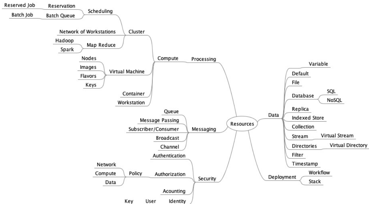
Figure 4: Resource view
