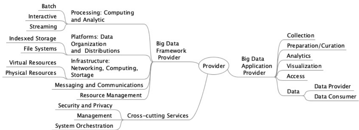
Figure 3: Provider view
