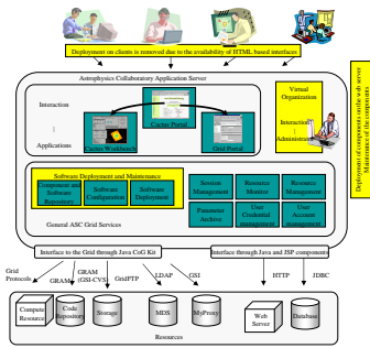
Fig. 3. Structure of the ASC application server showing the various components.
