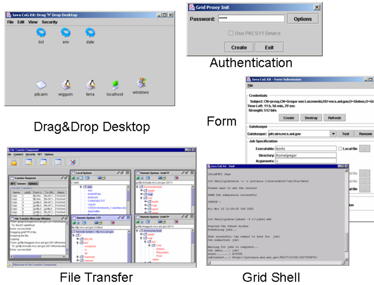
Fig. 1.7 Selected Java CoG Kit GUI components include convenient prototype interfaces to perform file transfer, job submissions, and service access while interfacing with Grid middleware.
