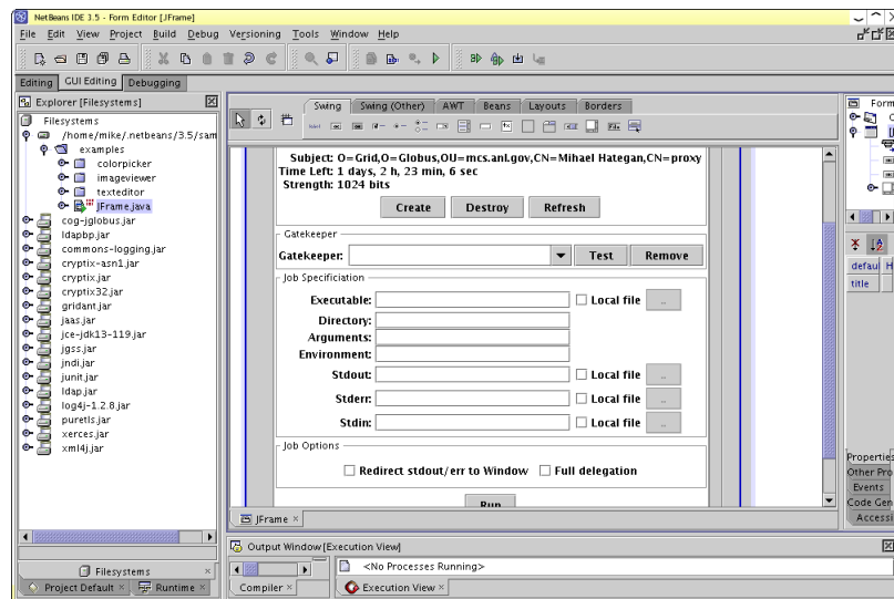
Fig. 1.6 The Java CoG Kit contains a number of JavaBeans that provides the next level of Grid middleware to develop simple, yet powerful components for Grid users. These beans can be reused in commodity interface Development environments (IDE), providing a GridIDE.
